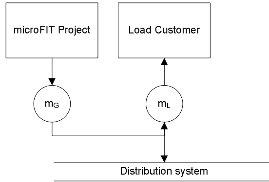
Figure 1b – Indirectly connected microFIT Project (in parallel)
